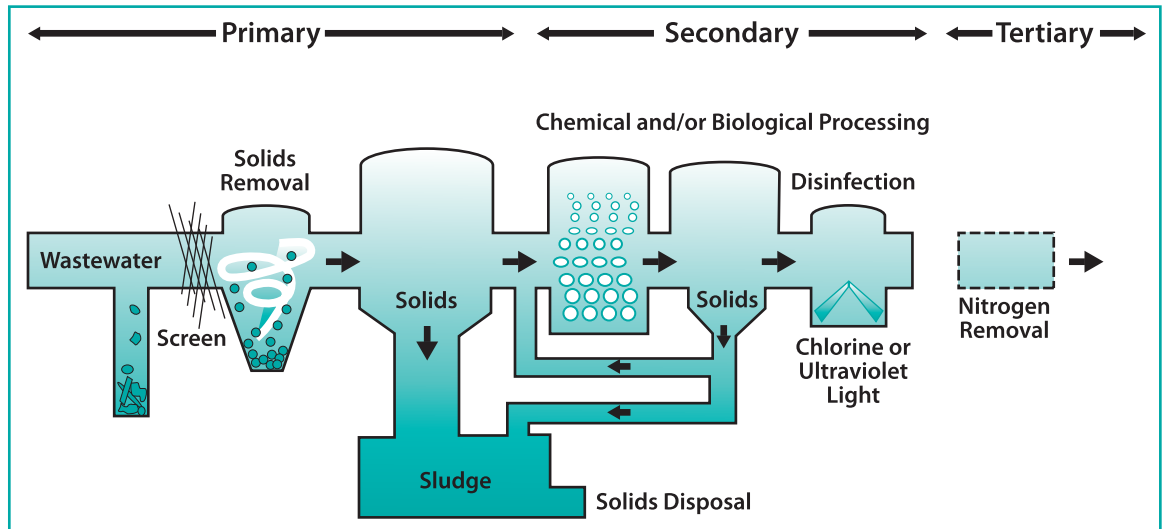
Typical reclaimed water treatment.
