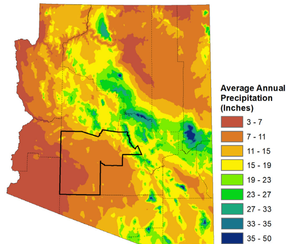
Mean Precipitation 1981-2010 (PRISM Climate Group 2016).
